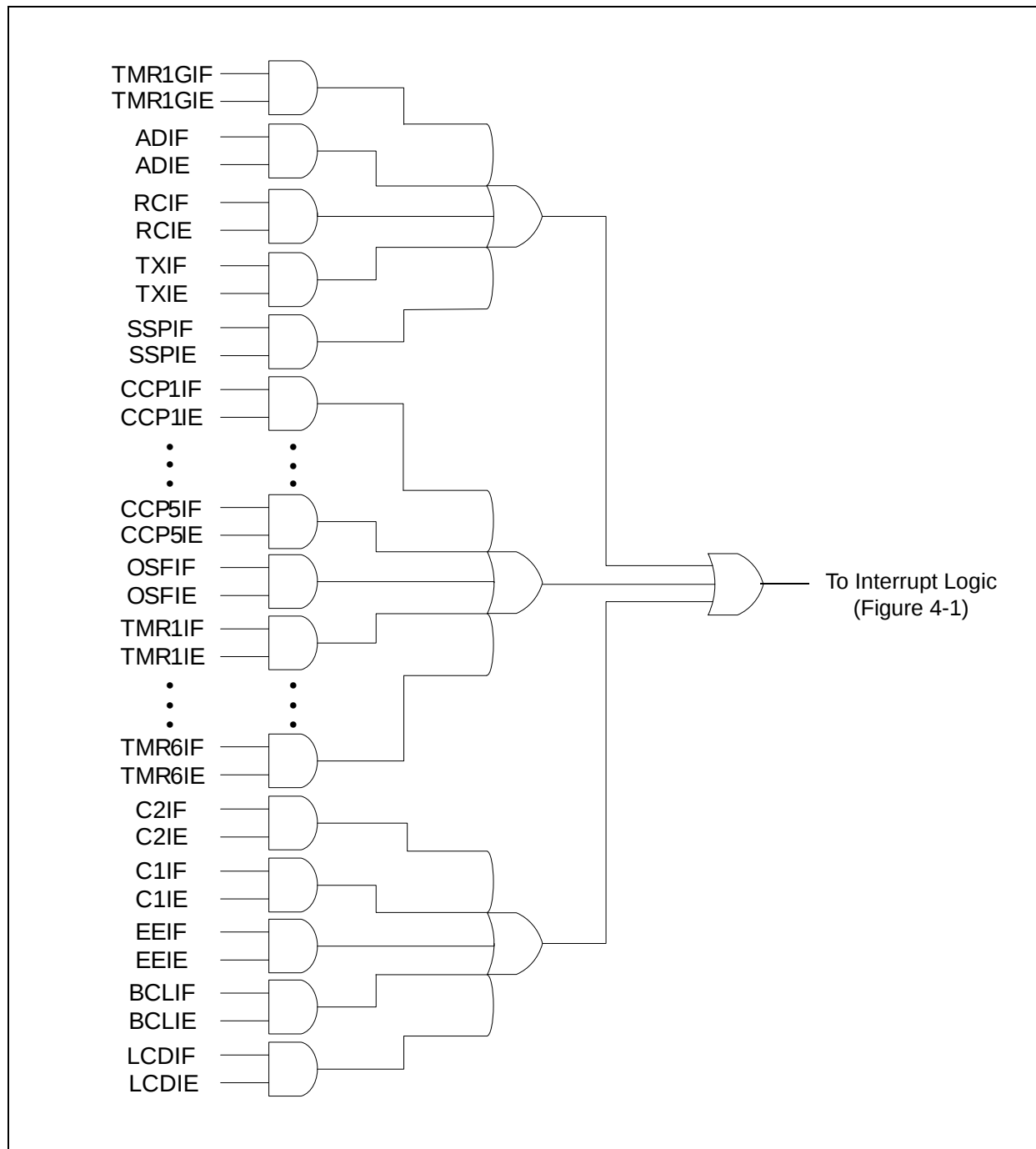
FIGURE 4-2: PERIPHERAL INTERRUPT LOGIC
