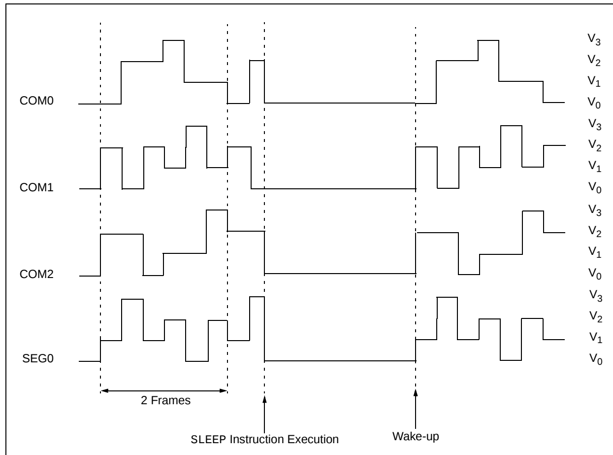
FIGURE 21-19: SLEEP ENTRY/EXIT WHEN SLPEN = 1
