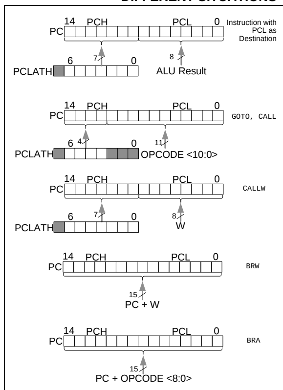
FIGURE 2-4: LOADING OF PC IN DIFFERENT SITUATIONS
